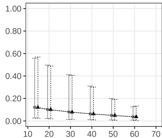
(C) RMSE
